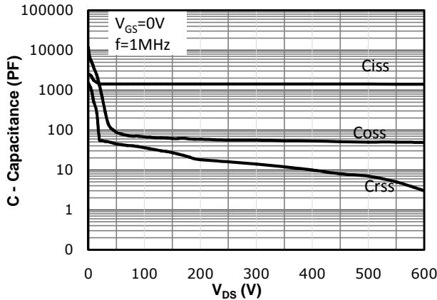
Fig 11: Capacitance Characteristics
